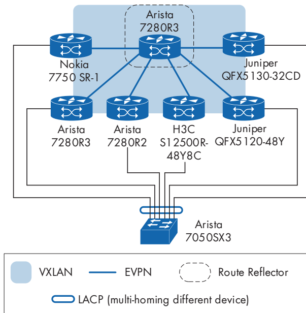
Figure 2: EVPN ESI Auto-Configuration
