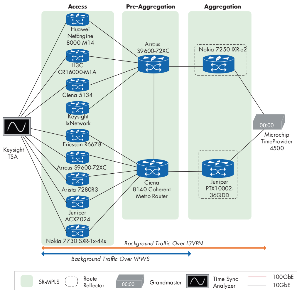
Figure 8: 5G xHaul over SR-MPLS
