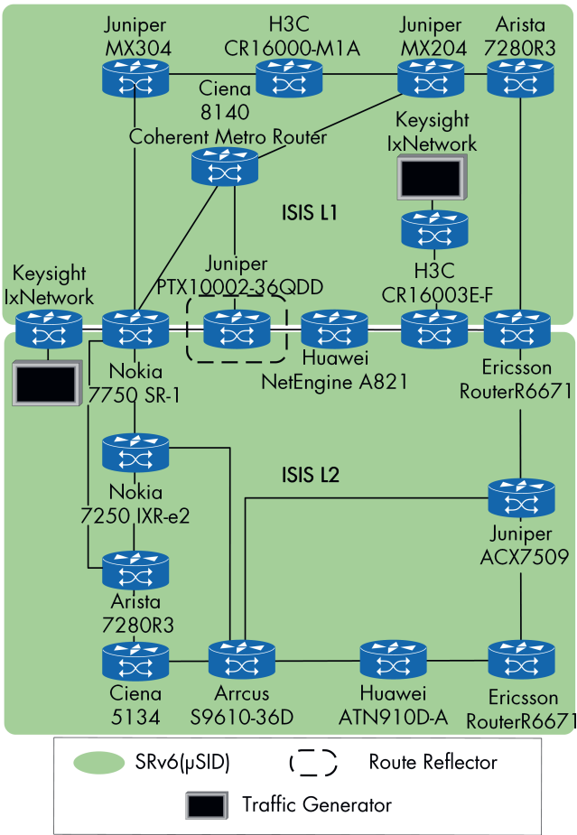
Figure 10: SRv6 Baseline Test Setup
