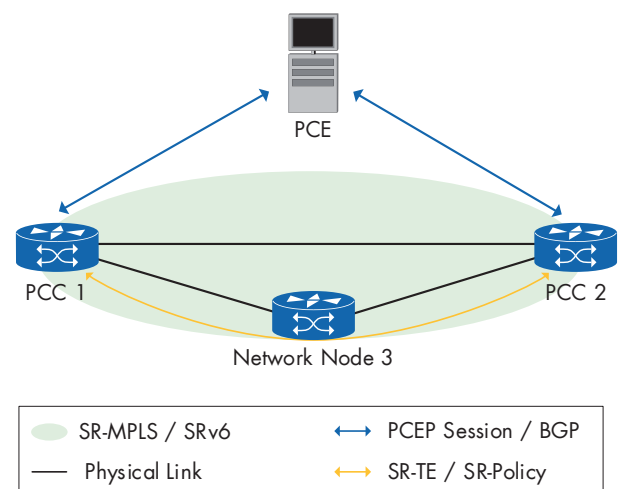
Figure 5: Path Computation Element Topology Overview
